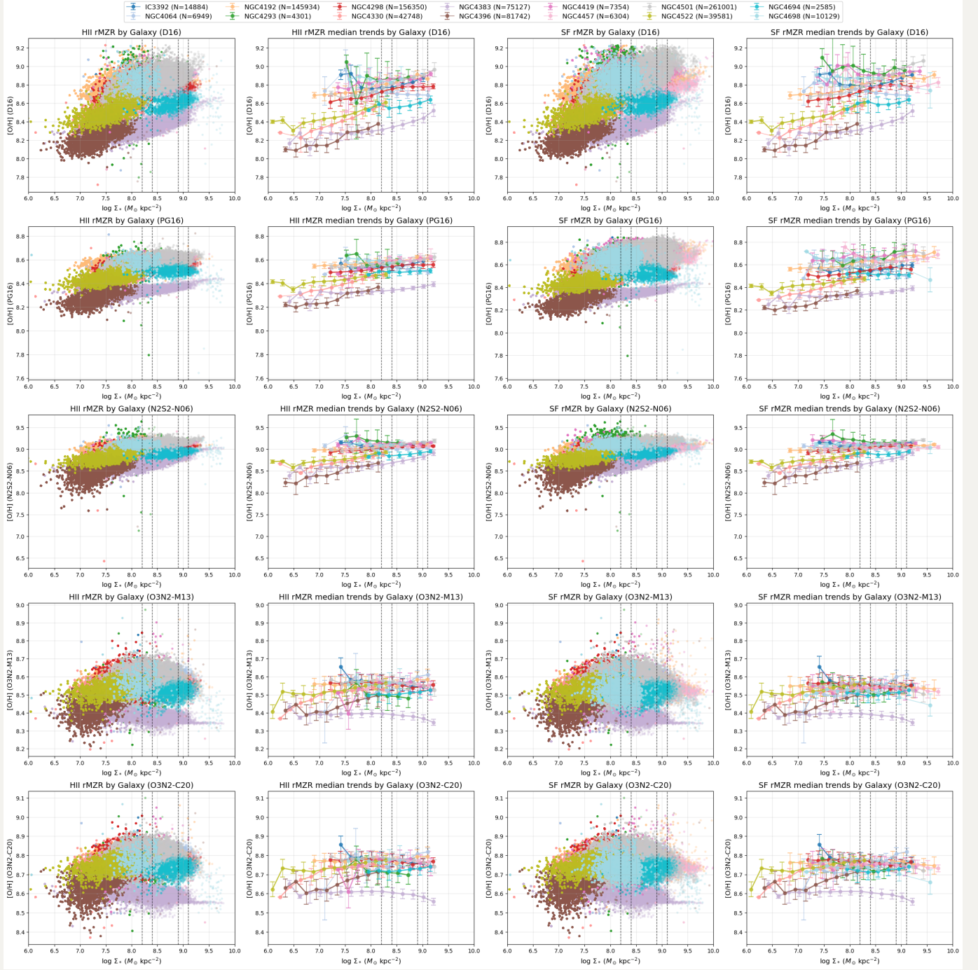
rMZR behavior by Galaxy: HII vs SF regions (Min 50 datapoints per bin, Adjacent bins only)
