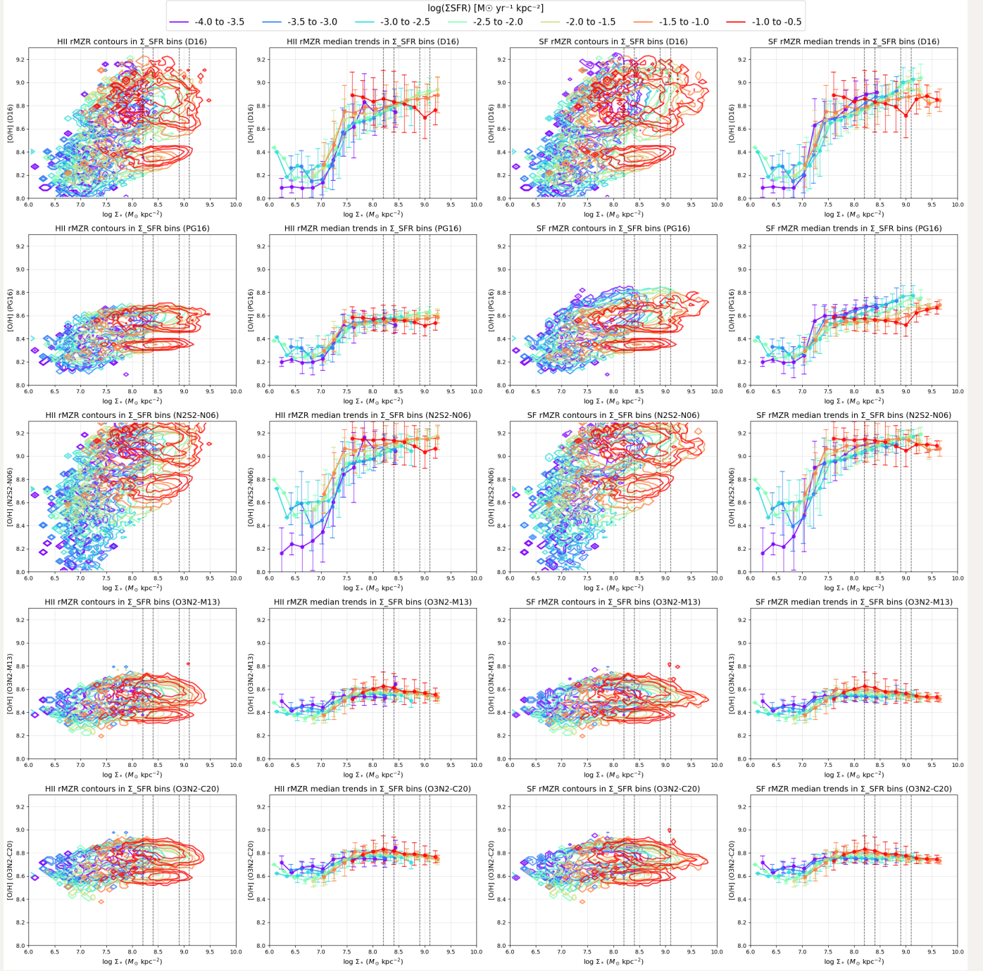
rMZR behavior in \Sigma_{\text{SFR}} bins: HII vs SF regions (Contour plots, Min 50 datapoints, Adjacent bins only)
