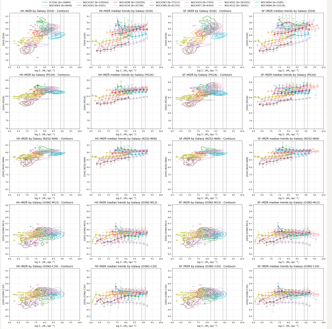
rMZR behavior by Galaxy: HII vs SF regions (Contour plots + Median trends)
